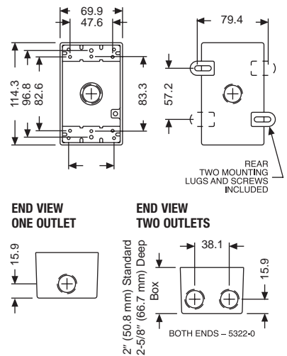
SINGLE-GANG BOXES: GENERAL DIMENSIONS
