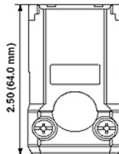
Dimensional Diagram
