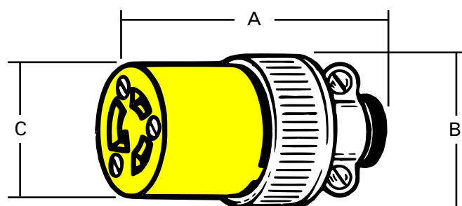
Connectors (2493 shown)
