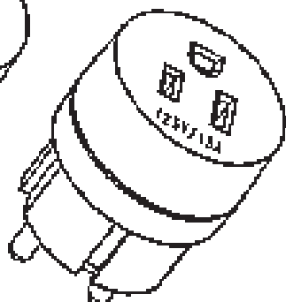
Catalog No. 114 Socket NEMA 5-15R (125V / 15A)
