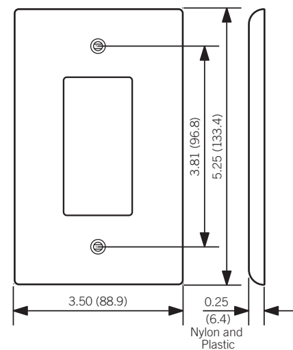
Oversized Single-Gang
