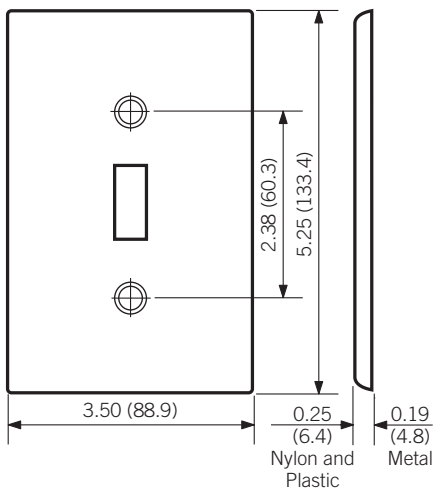
Oversized Single-Gang
